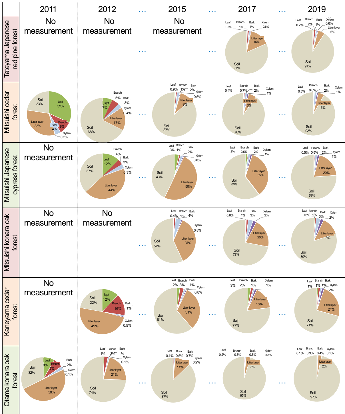
Figure 5 Percentage of Accumulated Radioactive Cesium Quantity by Section at Monitoring Sites from 2011 to 2019 (Note) Data are omitted for 2013, 2014, 2016, 2018.
