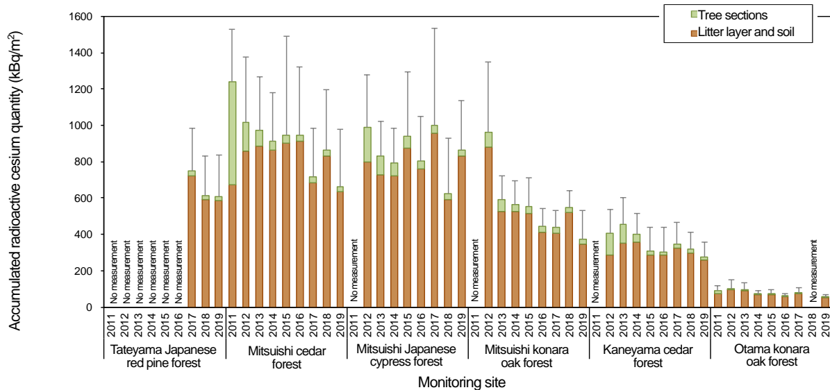
Figure 4 Changes in the Accumulated Quantities (Averages) of Radioactive Cesium for the Entire Forest from 2011 to 2019 (Fine lines indicate standard deviation)
