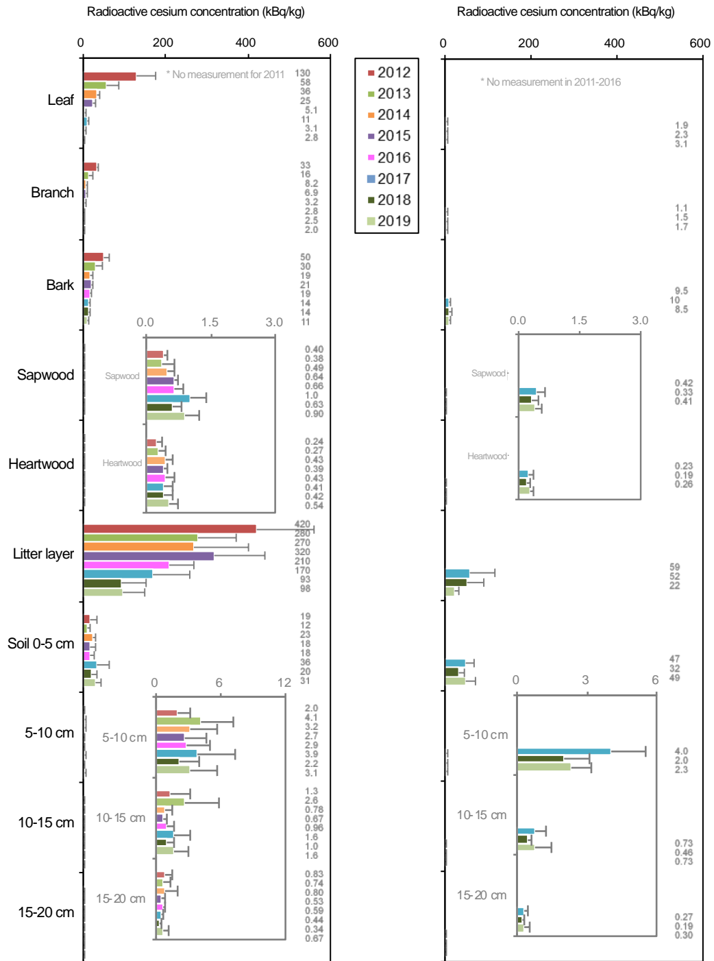
Figure 3 Changes in Radioactive Cesium Concentrations by Section at Each Monitoring Site (kBq/kg, average, 2 significant digits) (Fine lines indicate standard deviation. No measurement for Mitsuishi Japanese cypress forest in 2011 and for Tateyama Japanese red pine forest in 2011-2016.)
