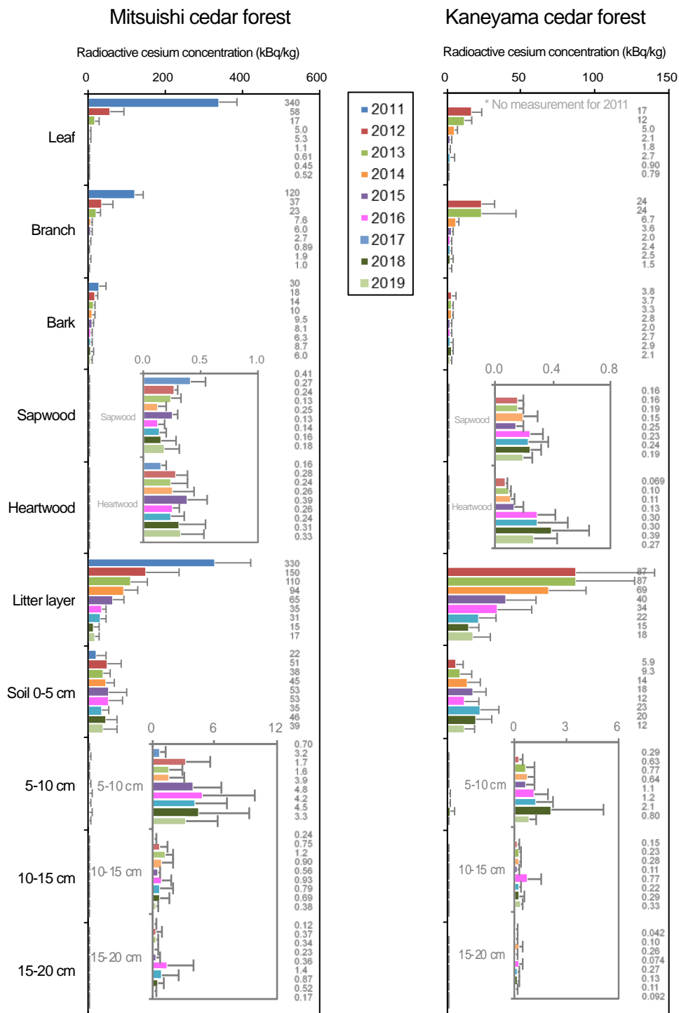
Figure 3 Changes in Radioactive Cesium Concentrations by Section at Each Monitoring Site (kBq/kg, average, 2 significant digits) (Fine lines indicate standard deviation. No measurement for Kaneyama cedar forest in 2011.)
