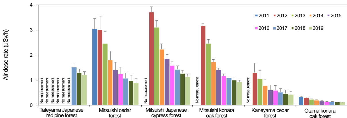
Figure 2 Changes in Air Dose Rates (Average) at Monitoring Sites from 2011 to 2019 (Fine lines indicate standard deviation.)
