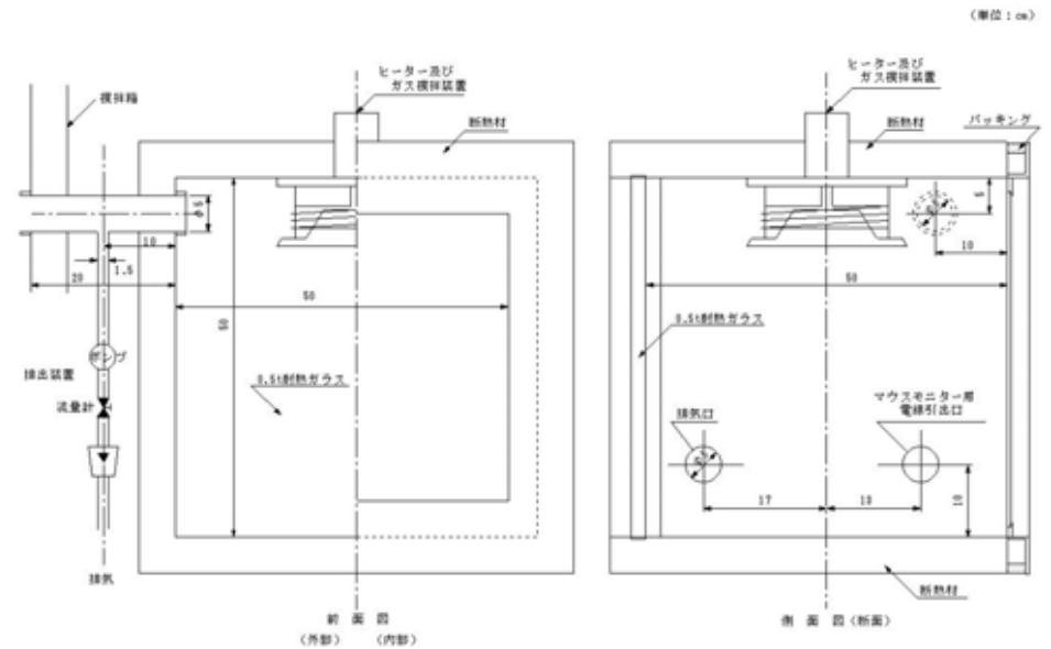
図9 披検箱
