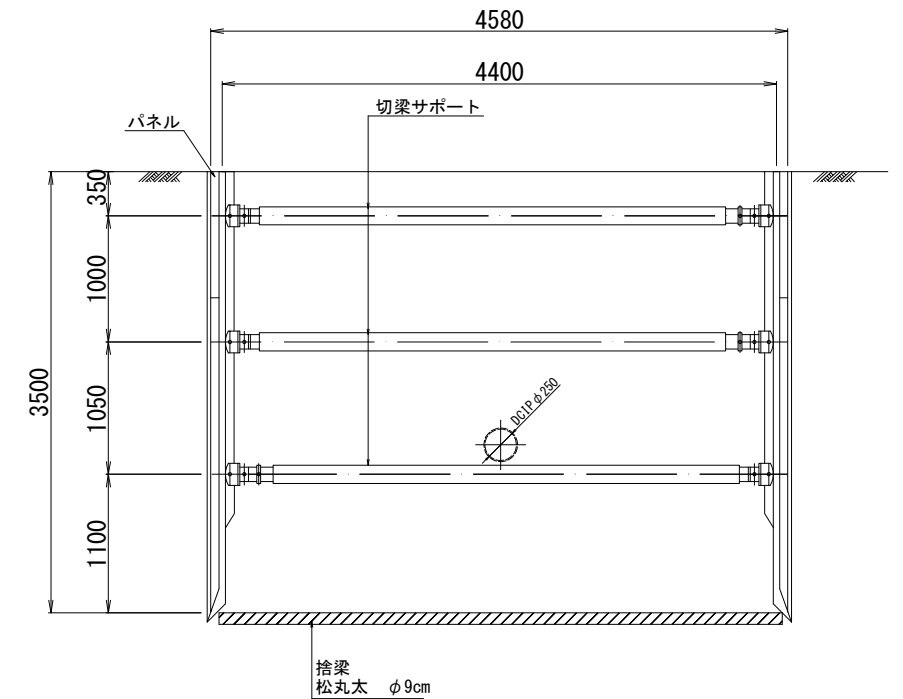
(No.0+5.27~No.0+11.37)
