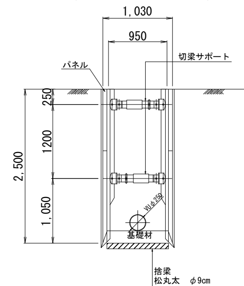
(No.0+11.37~No.0+13.00)
