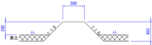
湛水畦畔 H=0. 0m (TK)
