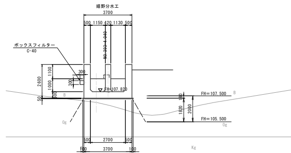
塘野分水工 (J-J断面) NO. 393+4.040
