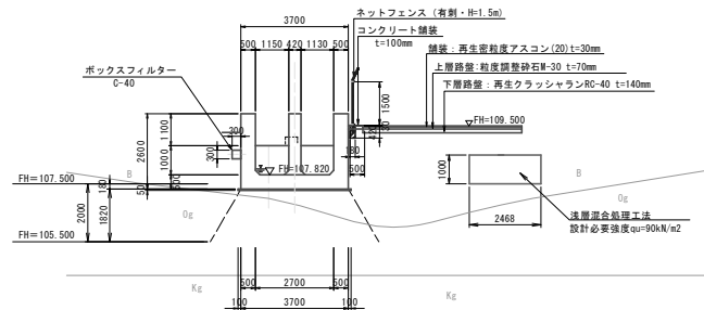
嬉野分水工 (I-I断面) NO. 393+2. 140
